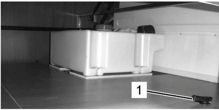
Fig. 102: Waste water tank (optional)
