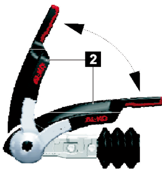
Fig. 7: Wear indicator
