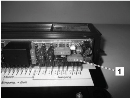
Fig. 75: 12 V-Emergency lighting
