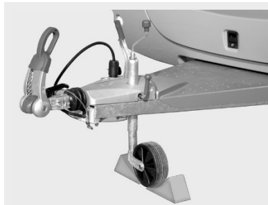
Fig. 173: Securing the support wheel
