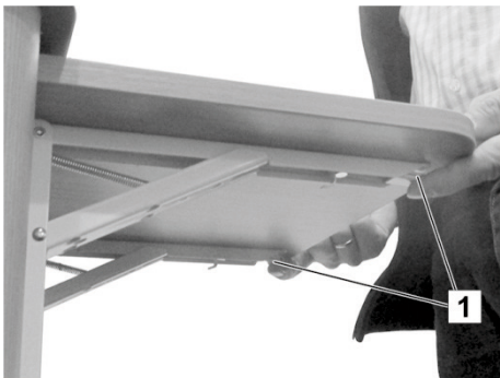
Fig. 167: Undoing the latching mechanism
