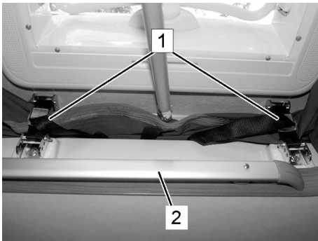
Fig. 151: Opening the pop-up roof
