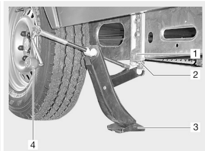
Fig. 176: AL-KO lift jack
