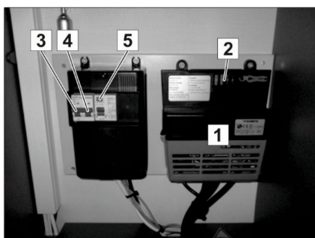
Fig. 74: Converter (power supply unit) (1) and cut-outs
