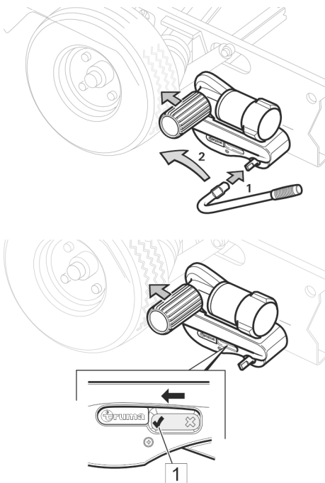
Fig. 17: Swivelling Mover smart M in
