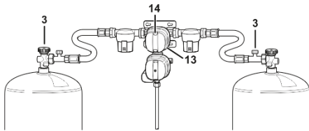
Fig. 118: Gas pressure regulator set
