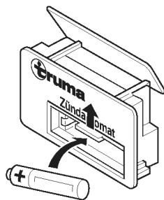
Fig. 135: Battery change
