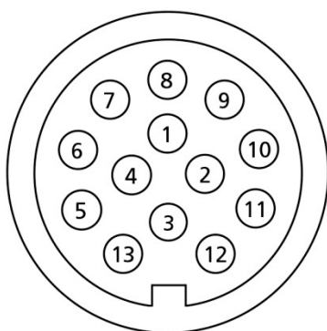
Fig. 2: 13-pole plug
