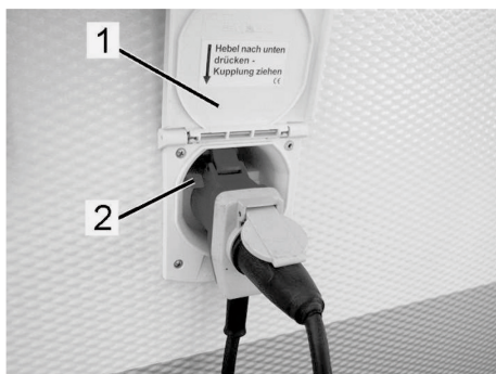
Fig. 73: Power connection
