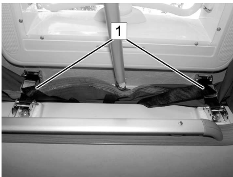
Fig. 155: Roof locking mechanisms
