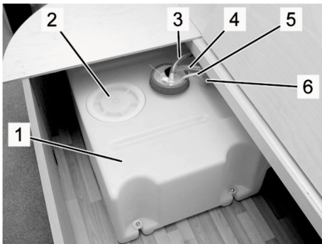
Fig. 98: Fresh water tank, example
